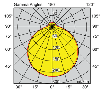
Ø350 23W @4000K
